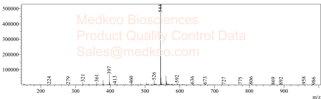
MS Spectrum
