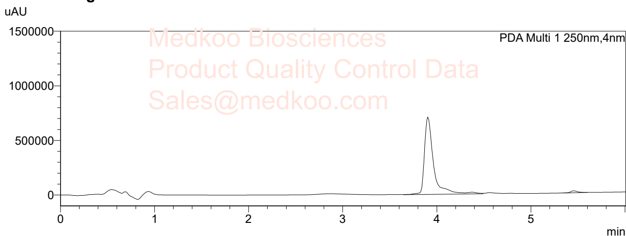
Peak Table
