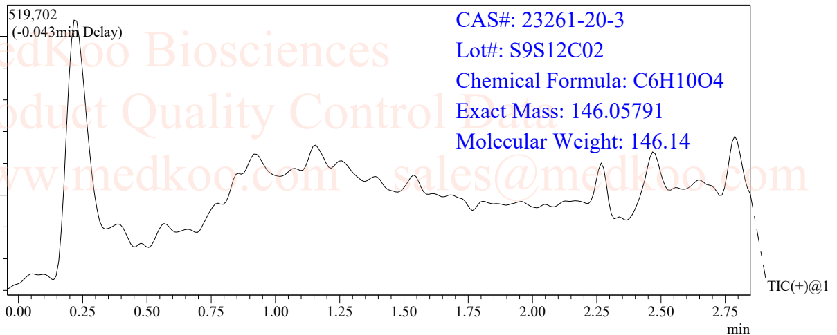
Mass Spectrum
