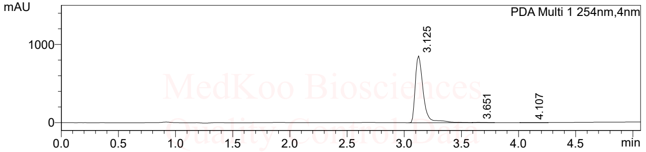
Peak Table
