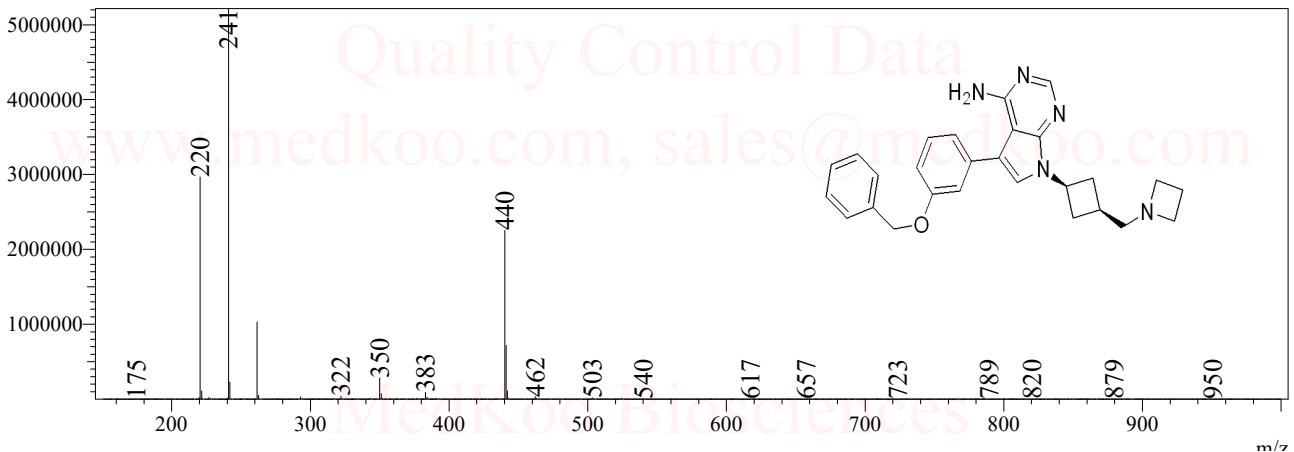
MS Spectrum
